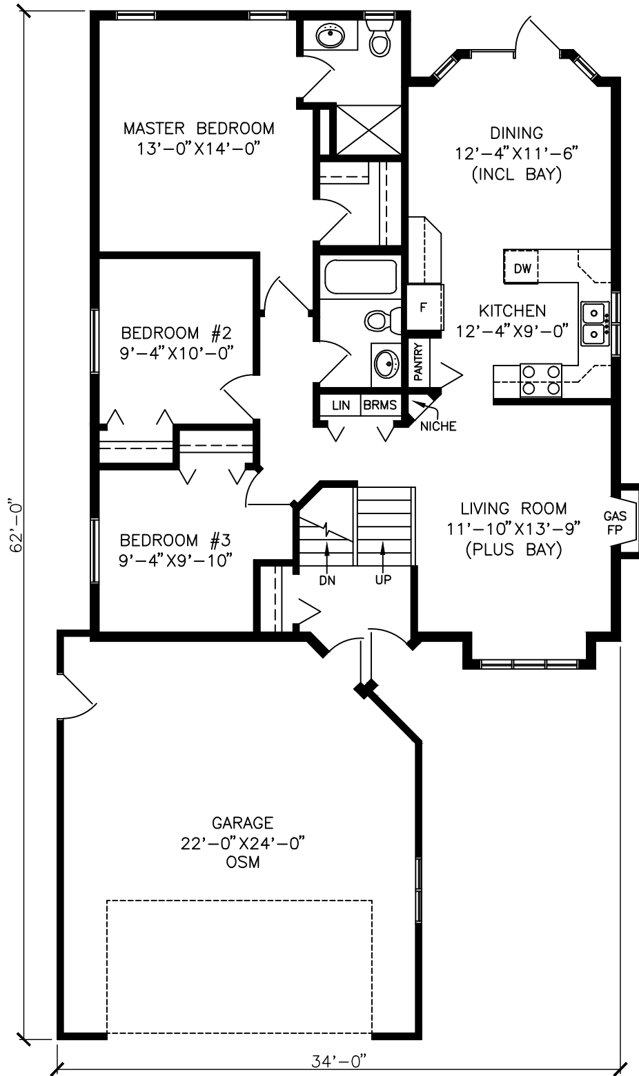
MAIN FLOOR PLAN 1203 SF
