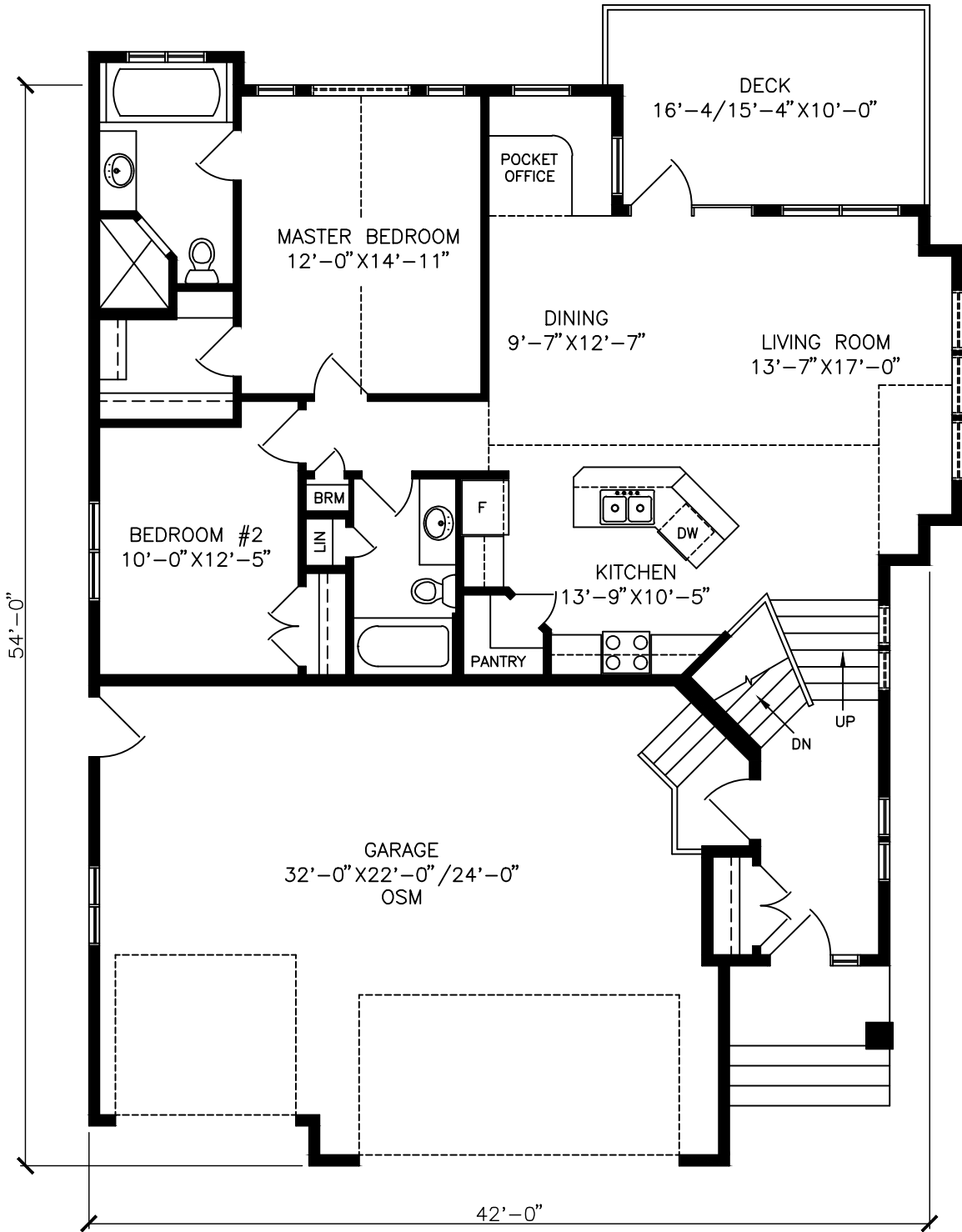
MAIN FLOOR PLAN 1311 SF
