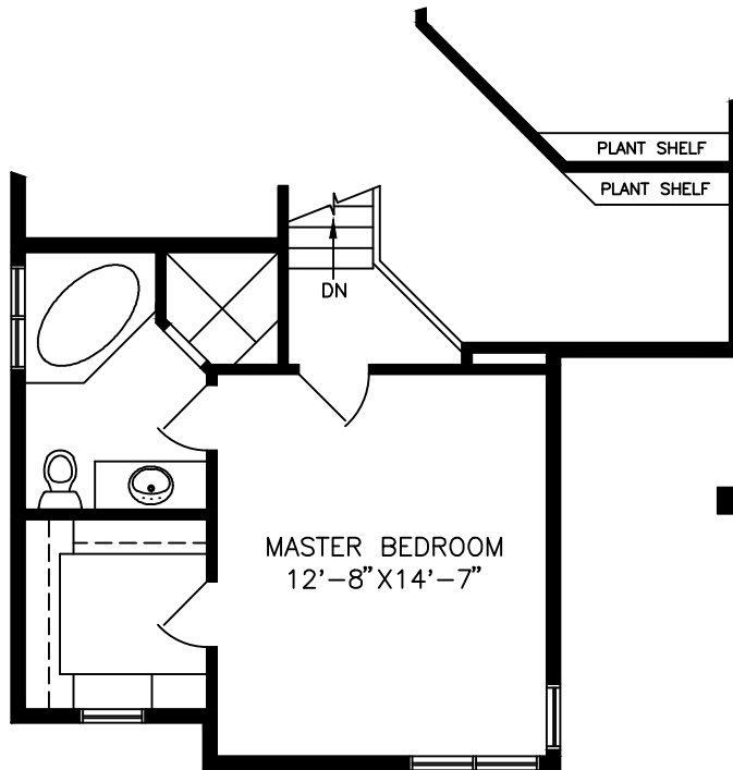
UPPER FLOOR PLAN 387 SF
