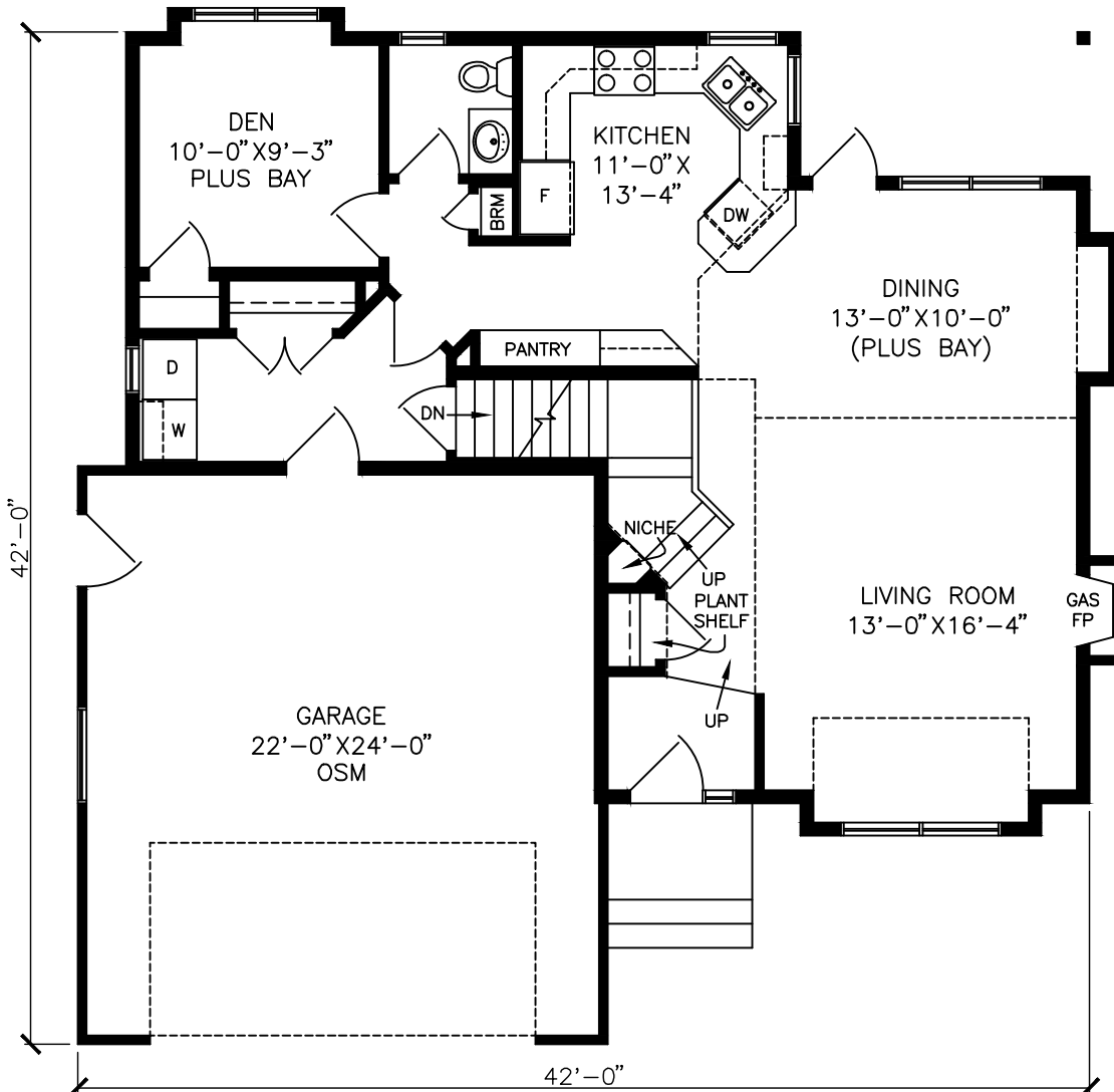
MAIN FLOOR PLAN 965 SF 1699 SF TOTAL
