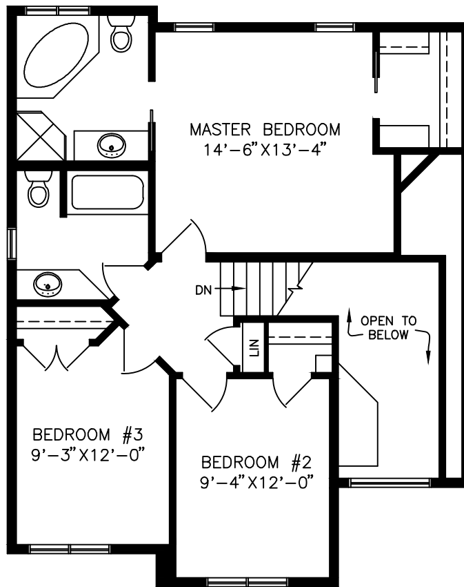
SECOND FLOOR PLAN 734 SF
