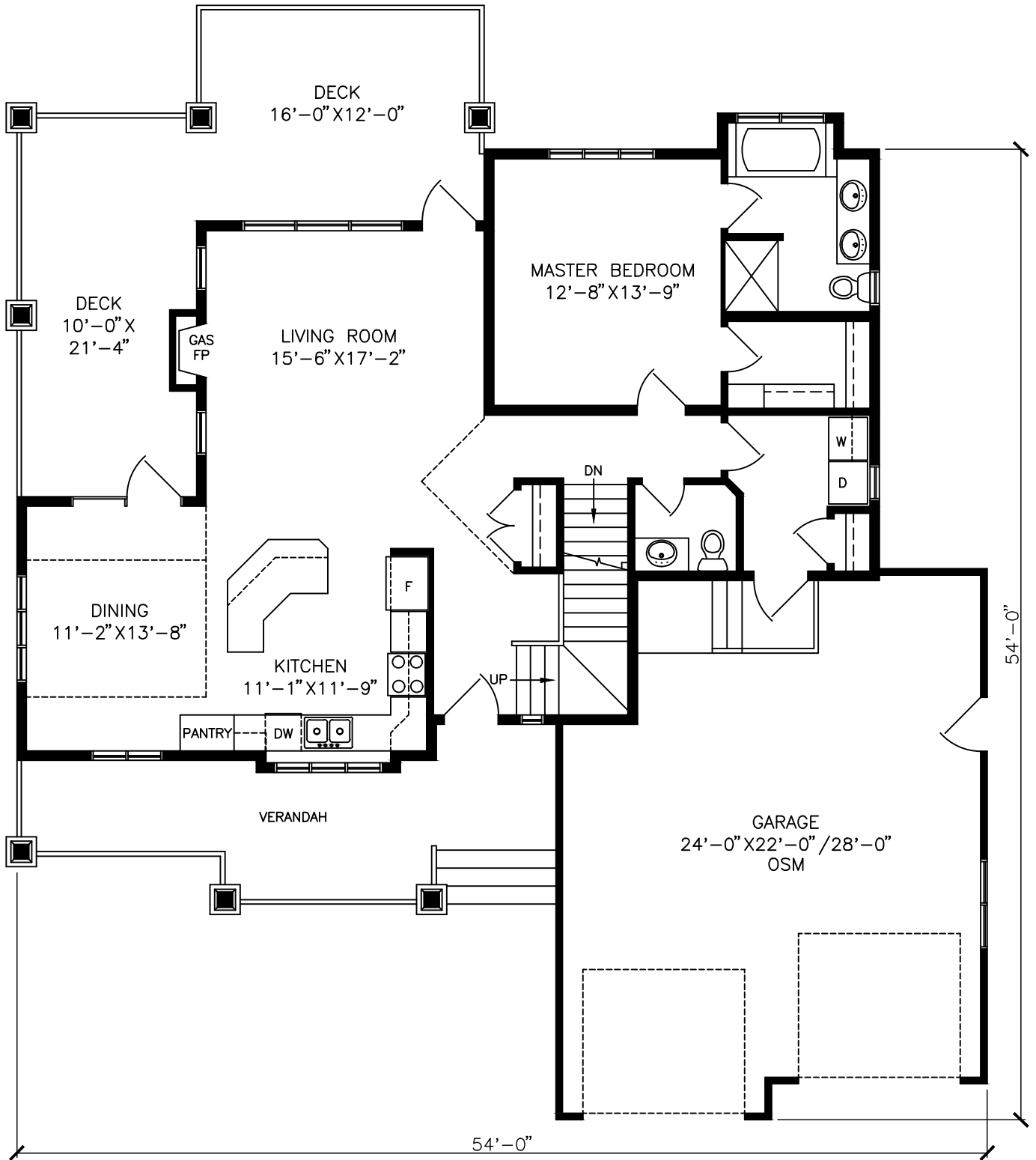
MAIN FLOOR PLAN 1232 SF 1753 SF TOTAL
