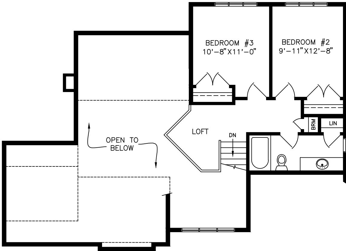
SECOND FLOOR PLAN 521 SF
