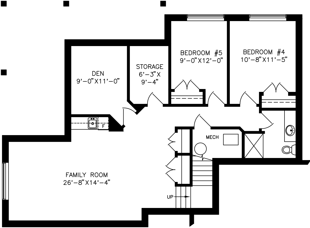
LOWER FLOOR PLAN 1218 SF
