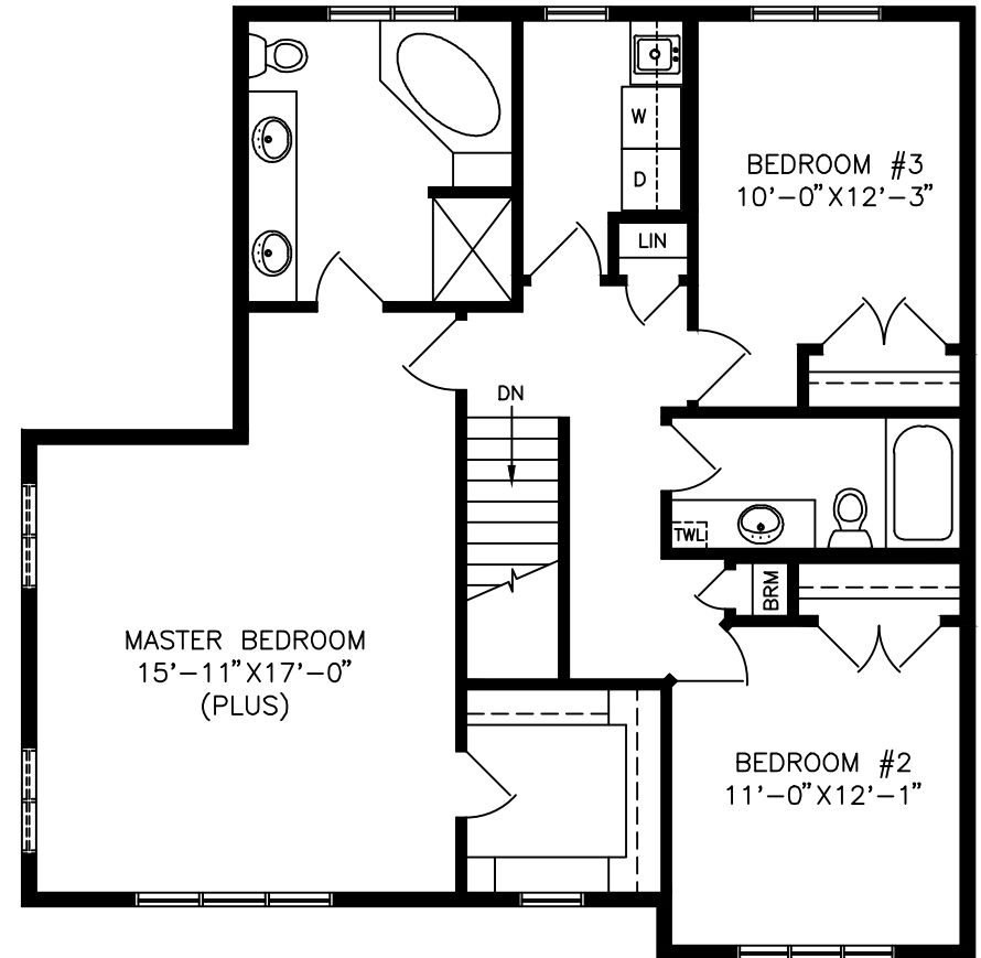
SECOND FLOOR PLAN 1120 SF
