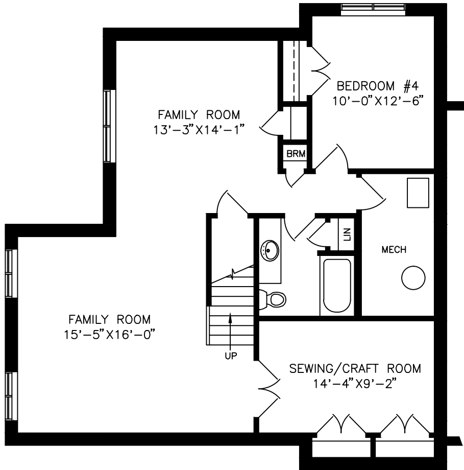
LOWER FLOOR PLAN 1144 SF
