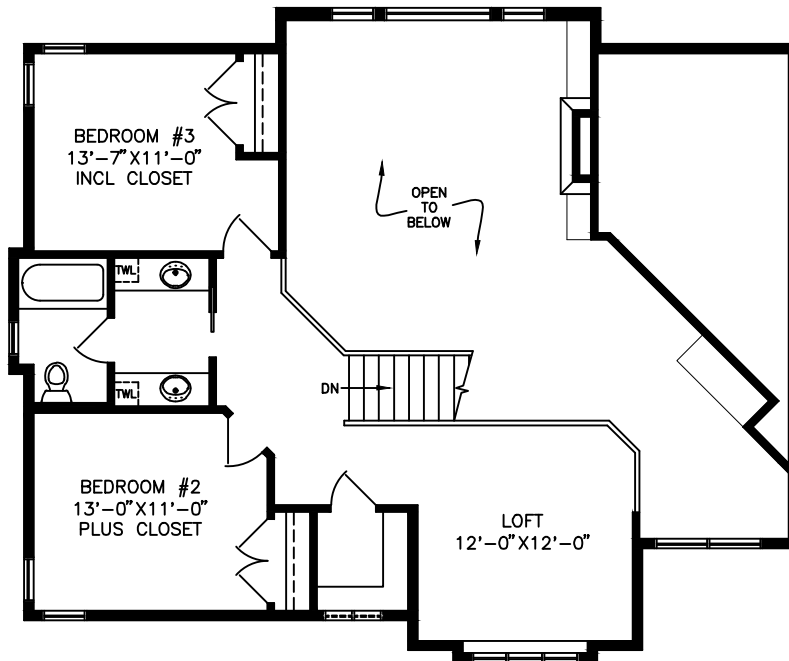
SECOND FLOOR PLAN 728 SF
