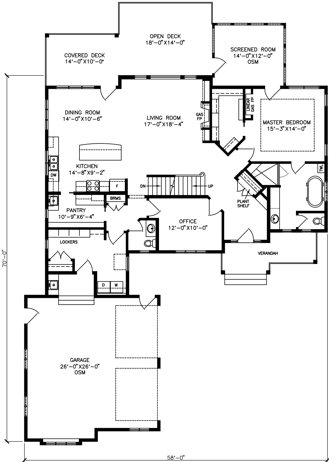
MAIN FLOOR PLAN 1793 SF 2521 SF TOTAL
