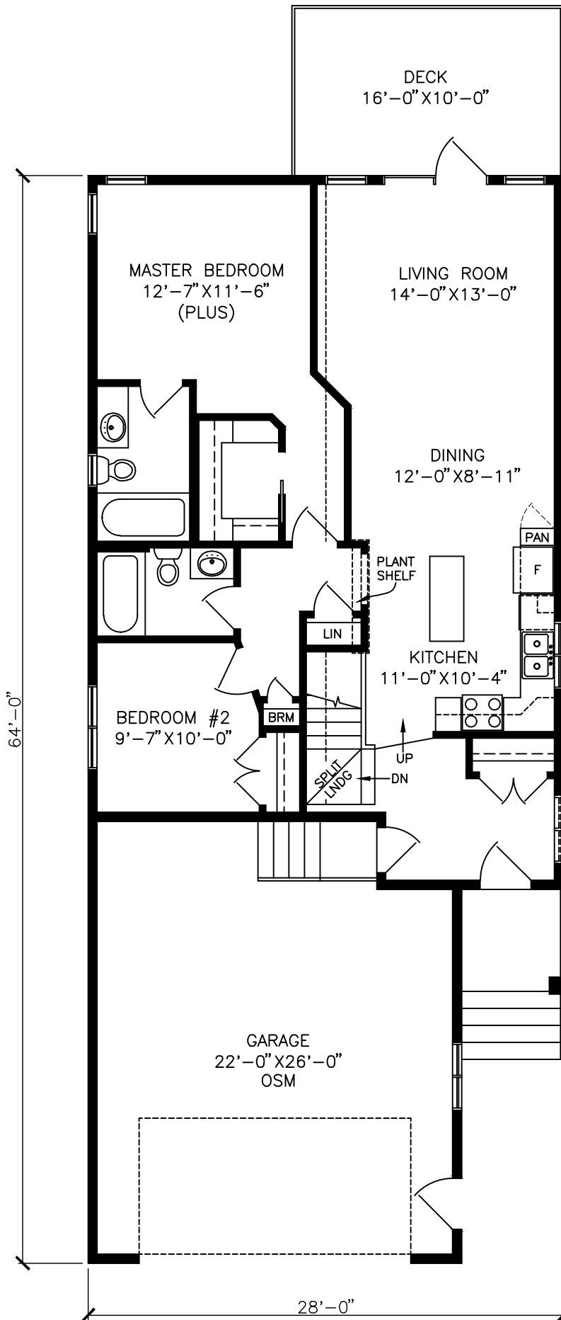
MAIN FLOOR PLAN 1108 SF
