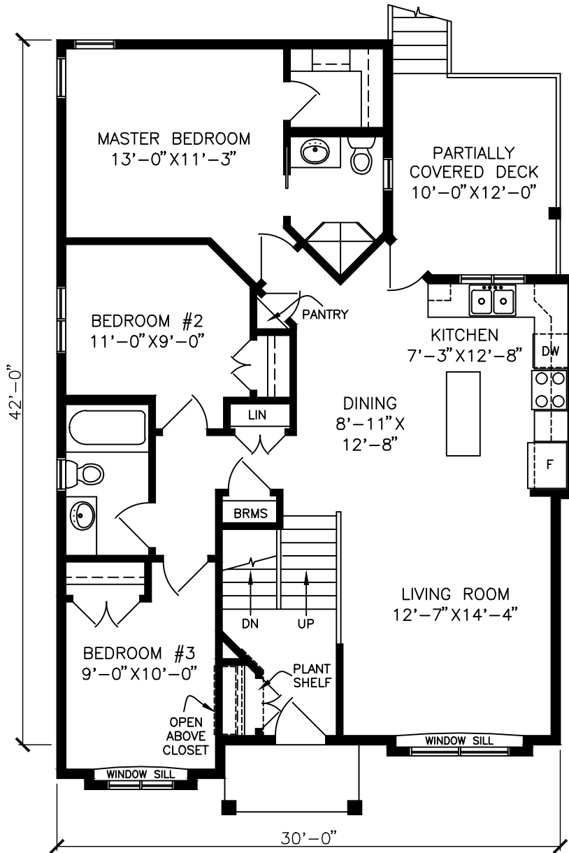
MAIN FLOOR PLAN 1156 SF
