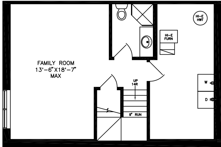
LOWER FLOOR PLAN 'B'
