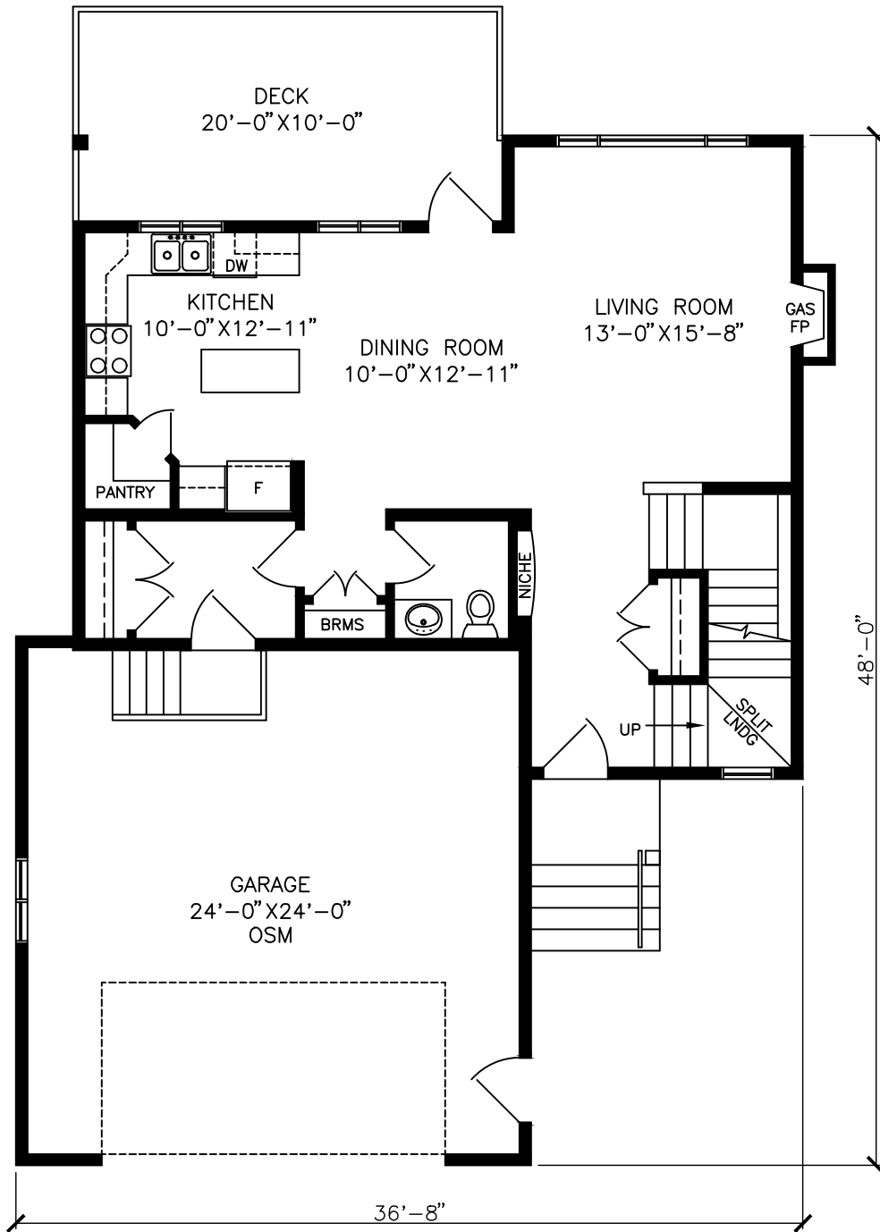
MAIN FLOOR PLAN 812 SF 1749 SF TOTAL
