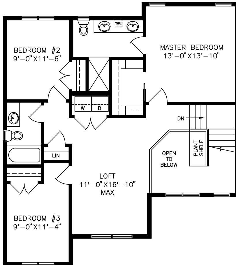
SECOND FLOOR PLAN 937 SF
